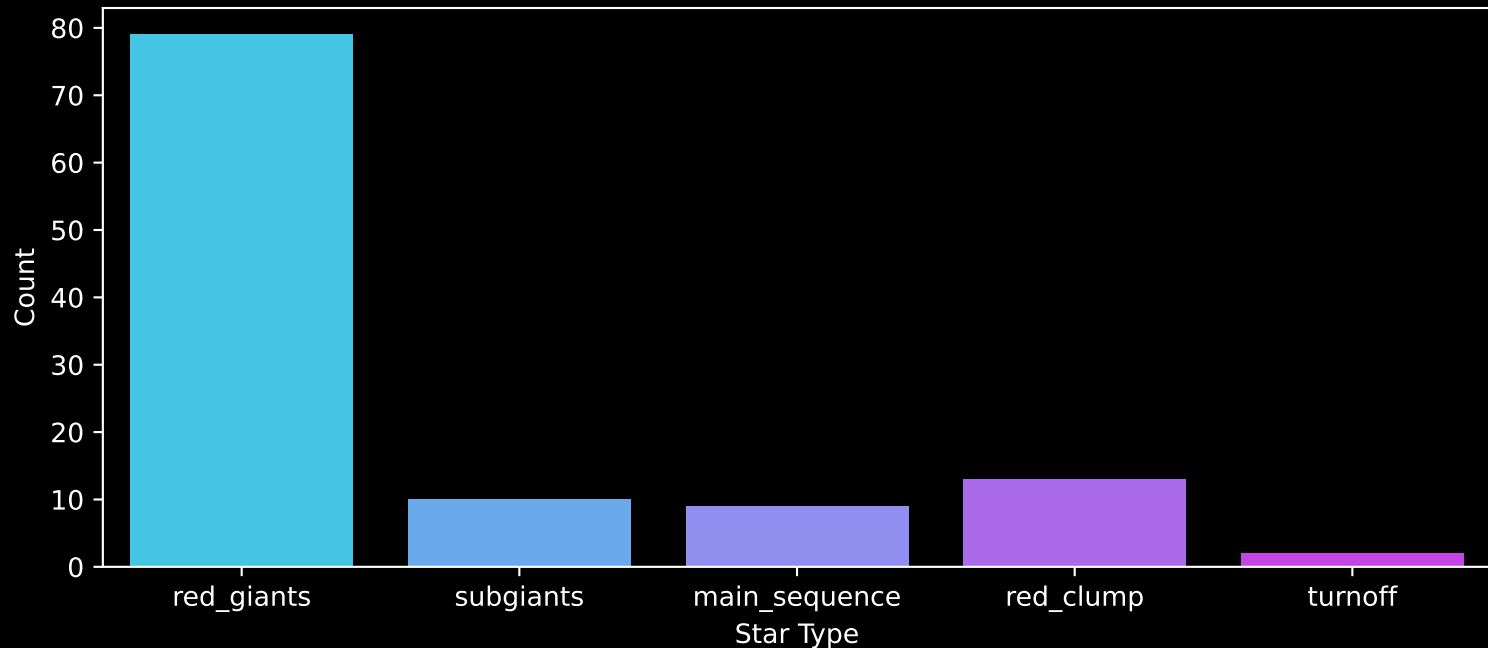
APOGEE DR17 Field: [012+00] Count plot of Star Type
